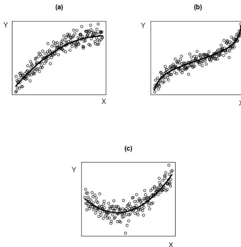
Figure 17. (a) A simple monotone relationship. (b) A monotone relationship that is not simple. (c) A simple nonmonotone relationship.
