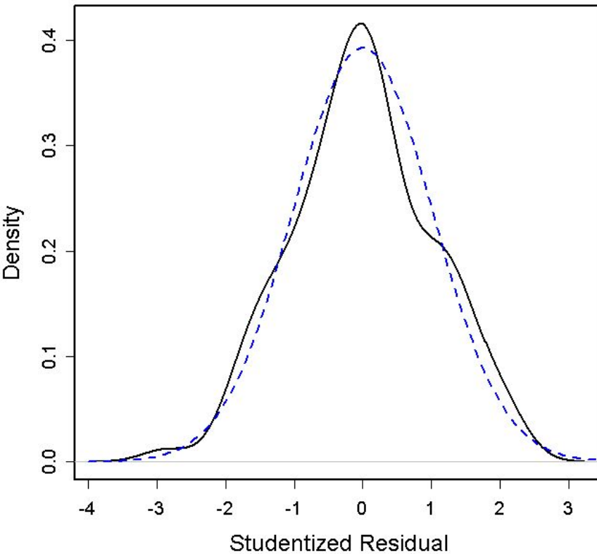
Density Plot to Assess Normality of Residuals
