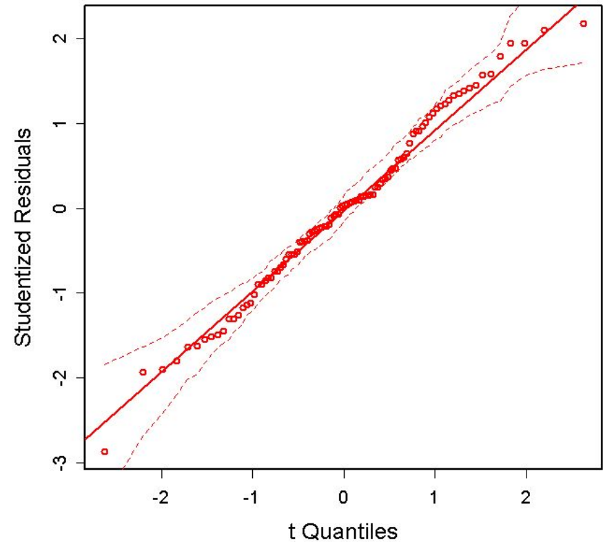
Quantile-Comparison Plot to Assessment Normality of Residuals
